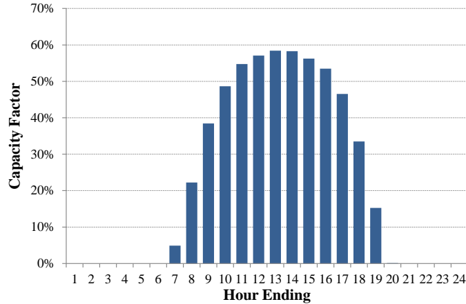
Figure 5 Average Hourly Solar PV Generation Profile (Texas, June-August period)
